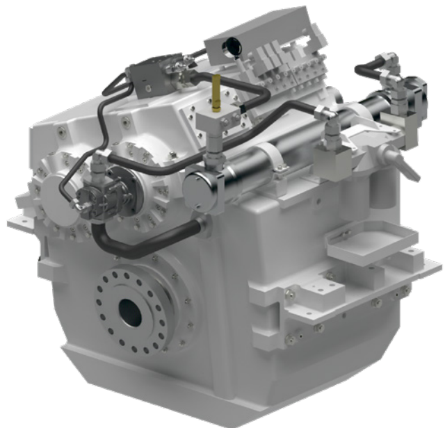
WSA 1542, propeller side
