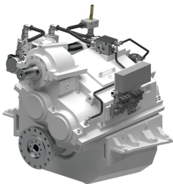
WWSFA 1542 U, engine and propeller side
