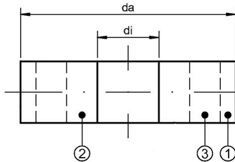
Figure 2 zones for punched disks
