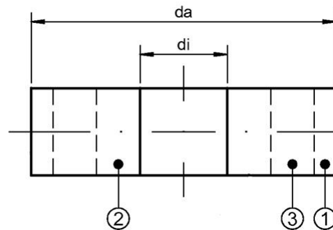
Figure 2 Zones for punched discs / rings
